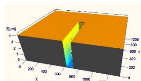
Fig. 8 Measurement of 4 \mu m step height
