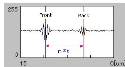
Fig.2 Interferogram of a transparent object
