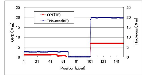
Fig.6 Profile data of plastic films by KF and TF method
