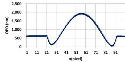
Fig.3. Optical path difference profile
