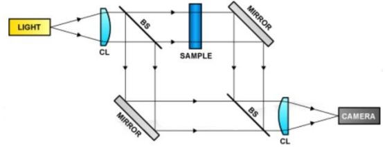
Fig.1. Mach-Zehnder interferometer
