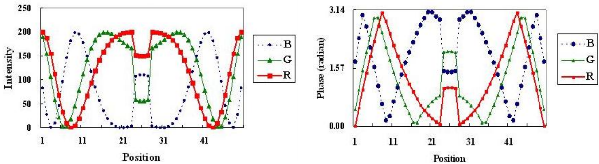
Figure 9. Observed intensities and phase profiles in the second step.
