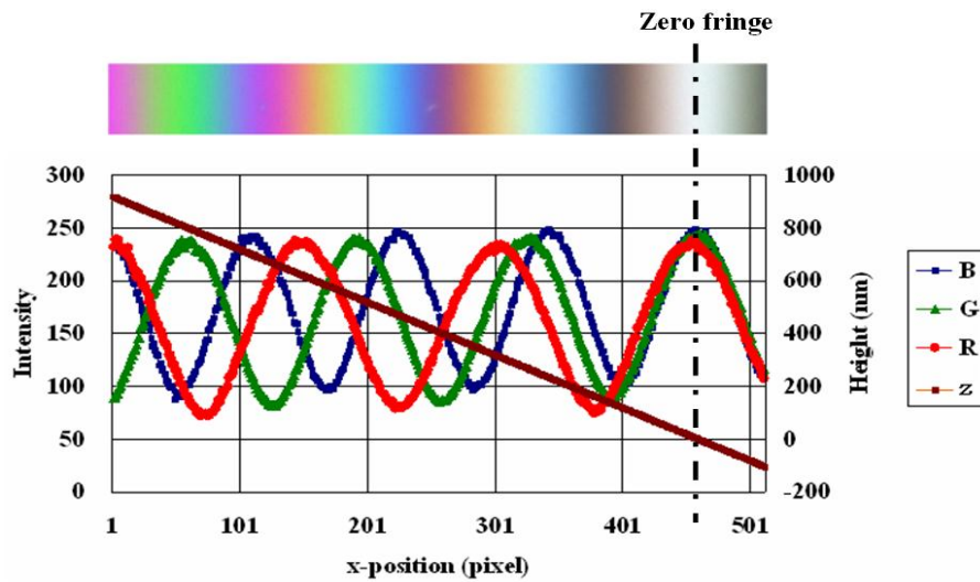
Figure 2. Relation between color and surface height in three-wavelength interferometry.
