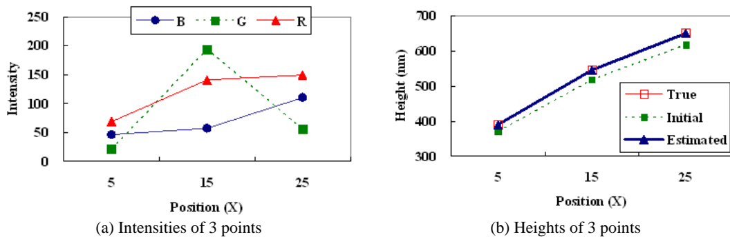
Figure 8. Observed intensities and the estimated height by the 3-point fitting.
