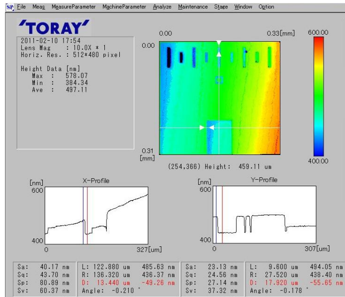
Figure 16. Estimated heights at 512×480 pixels by the ACOS method. The upper panel is a 3-dimensional map, and the lower graphs show x- and y-profiles.
